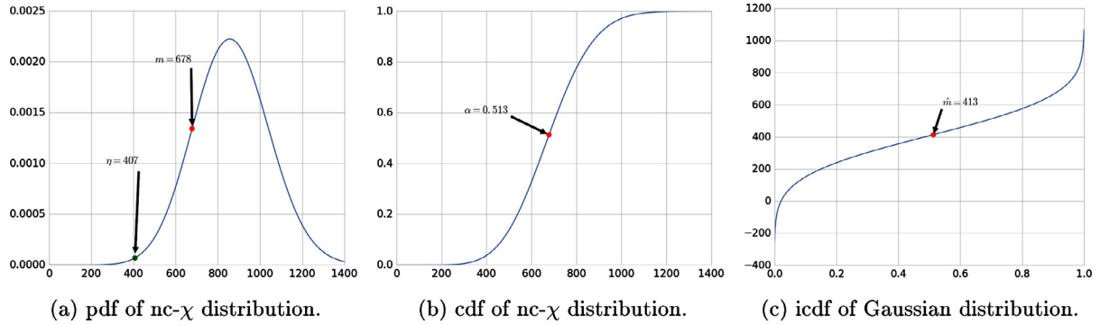
Fig. 3. A synthetic example of the stabilization algorithm. (a) Given a noisy value m = 678 observed in a nc- \chi distribution with N = 4 and \sigma_G = 200 , the underlying value is estimated as \eta = 407 . (b) The associated probability in the nc- \chi cdf with \eta is \alpha = 0.513 . (c) thus giving from the inverse cdf of a Gaussian distribution with mean \mu = 407 and standard deviation \sigma_G = 200 a new noisy value \hat{m} = 413 .
