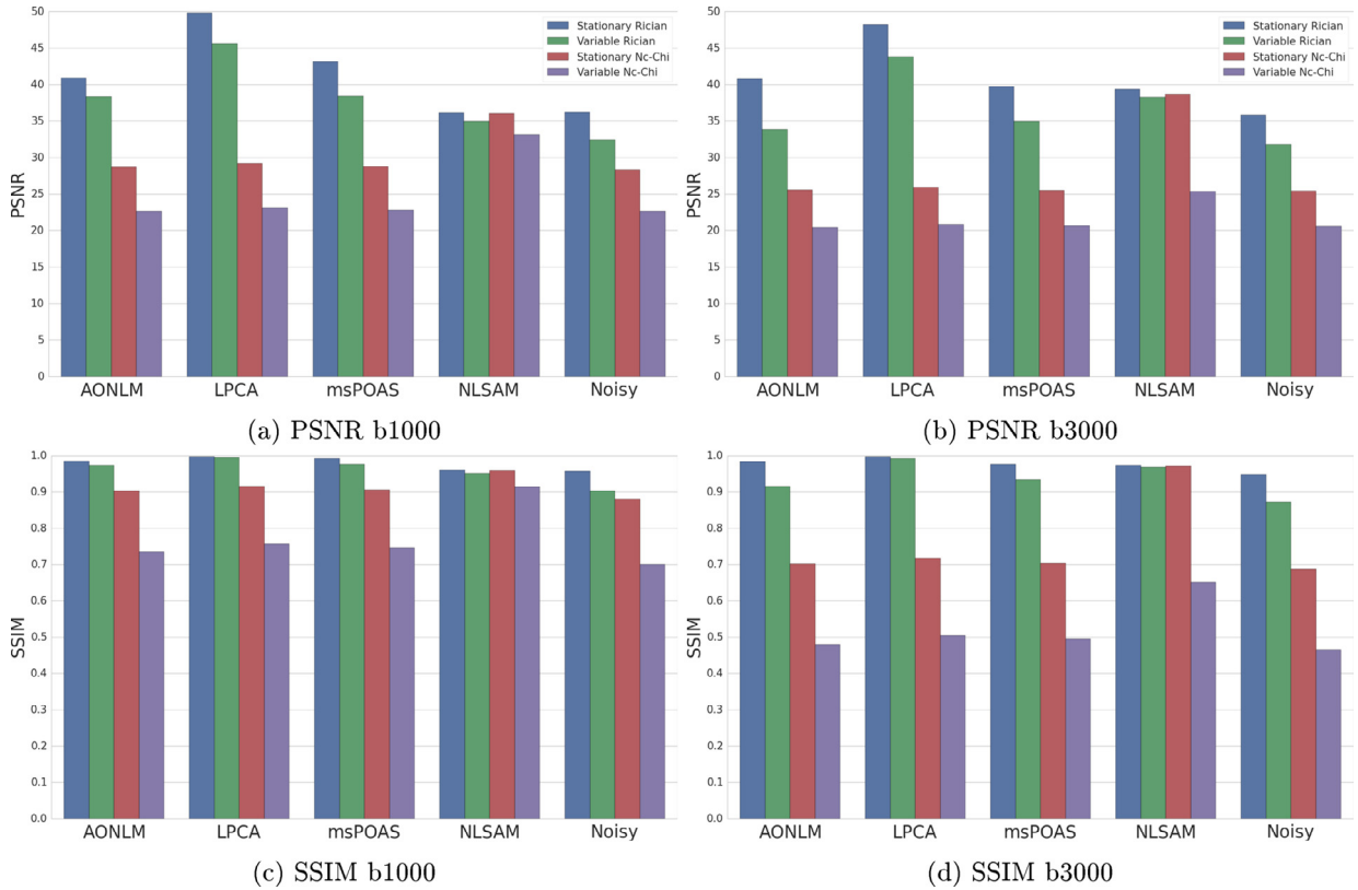
Fig. 7. PSNR and SSIM metrics for the SNR 10 stationary and SNR 15 spatially variable noise cases datasets. All methods can correct the stationary and spatially varying Rician noise case to some extent while only our NLSAM algorithm has the best performance for the nc- \chi noise case, especially for the spatially varying noise case.
