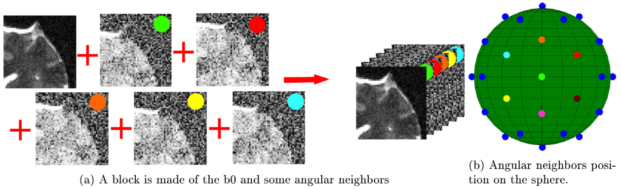
Fig. 1. (a) A 3D block is made by stacking along the 4th dimension the b_0 , a DWI and its angular neighbors, which share similar structure, but under a slightly different noise realization. (b) Disposition of equidistant angular neighbors on the sphere.
