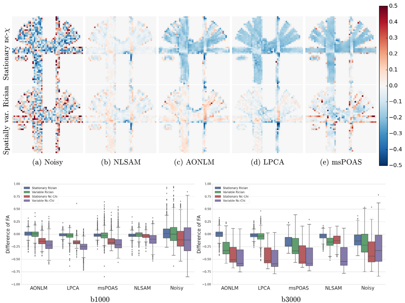
Fig. 8. Boxplot of the difference in FA for the synthetic datasets at b1000 (left) and b3000 (right). The whiskers show 1.5 times the interquartile range ( 1.5 \times \text{IQR} ), where outliers are plotted individually. The bars represent the first quartile, the median and the third quartile. No method performs well on the nc- \chi b3000 spatially varying noise case, which is the hardest test case. NLSAM overall produces less error or is equal to the other methods, but has a lower bias in the FA error along noise type. FA difference for the phantoms stationary nc- \chi SNR 10 and spatially varying Rician SNR 15 b1000 datasets. Blue values denote underestimation while red values show overestimation of the FA. Top : Stationary nc- \chi noise. NLSAM is less biased than the other methods in large, homogeneous regions, while the compared methods produces more underestimation for the nc- \chi case. Bottom : Spatially variable Rician noise. While being a harder case than the SNR 10 dataset since it varies from SNR 5 to 15, all methods adapt themselves to some extent to the varying noise profile.
