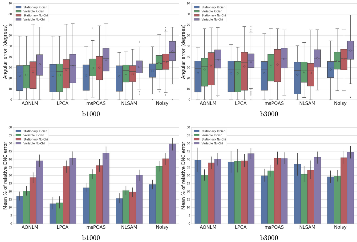
Fig. 9. The mean relative percentage of DNC error for the synthetic datasets. The bar represents the 95% confidence interval on the mean as computed by bootstrapping. The DNC error is the number of peaks found in excess or missing in each voxel with respect to the noiseless dataset. Boxplot of the angular error in degrees on the synthetic datasets, where the dot represents the mean angular error. A low angular error means that the extracted fODFs peaks are aligned with the noiseless dataset extracted peaks.
